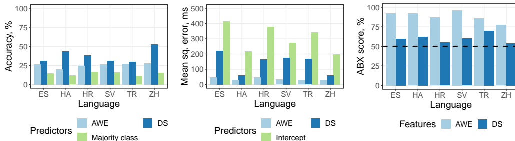
Figure 3: ABX scores in the task with words A and X matched on word duration, and B and X on speaker identity.
